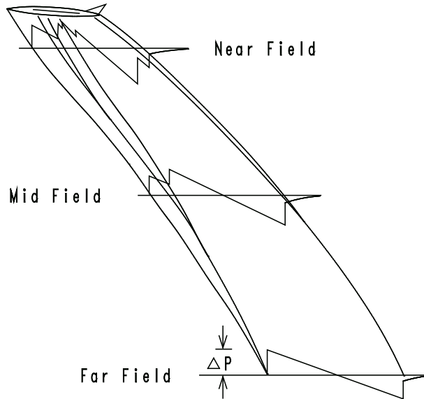
Figure C-5. Sonic Boom Generation and Evolution to N-Wave
